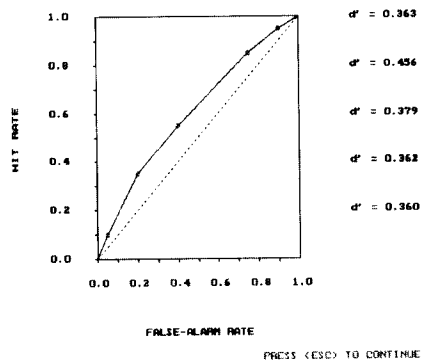
Figure 4. Receiver operating characteristic (ROC) curve provided by the SDT-SP, corresponding to hypothetical data from Table 4.
