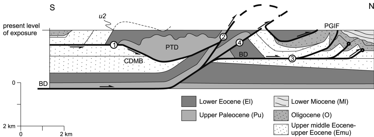
Figure 3. Northern balanced cross-section (modified from Torres Carbonell et al. , 2008b). Numbers indicate thrust sequence. BD: Basal detachment; CDMB: Campo del Medio backthrust; PTD: Punta Torcida deformation; PGIF: Punta Gruesa imbricate fan. See location in figure 1.
