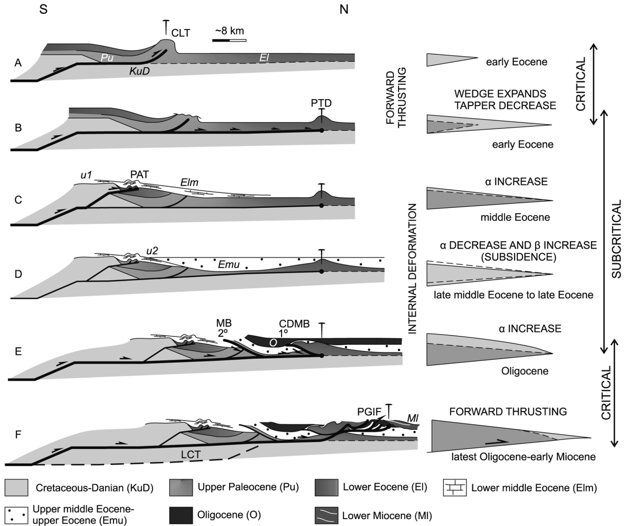
Figure 4. Schematic diagram showing evolution of the orogenic wedge in relation to critical taper, see text for explanation. Heavy lines mark active faults at each stage. Abbreviations are the same as for figures 2 and 3. Schematic wedges are light shaded light for geometry at each stage, while dark shading indicates previous stage geometry. Scale and angular relationships are approximate.
