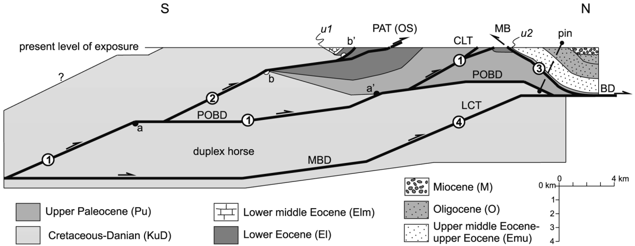
Figure 2. Southern balanced cross-section. Considering its position before the Fagnano fault offset, this cross-section is located 15 km southwards from the northern cross-section. Numbers indicate thrust sequence. Pin line is active only for times of thrust 4. POBD: Paleocene to Oligocene basal detachment; MBD: Miocene basal detachment; CLT: Cabo Leticia thrust; PAT (OS): Punta Ancla thrust (out-of-sequence); MB: Malengüena backthrust; LCT: La Chaira thrust; BD: basal detachment. See location in figure 1.
