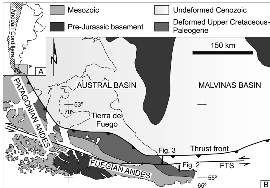
Figure 1. Location map of Tierra del Fuego in South America (A) and its main geological features (B). The trace of the cross-sections of figures 2 and 3 are indicated. FTS: Fagnano transform system.
